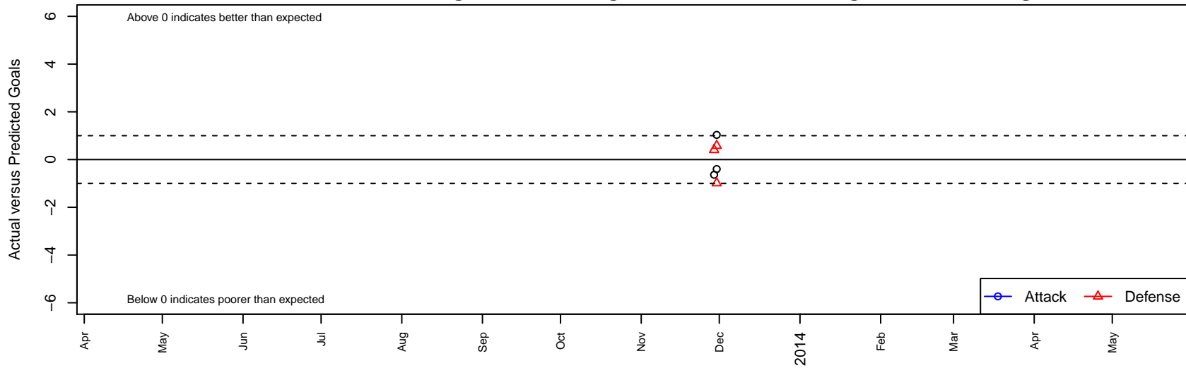
Odyssey 96 TXN B95 Dots are actual minus expected GF (blue circles) and GA (red triangles). Blue line is smoothed change in attack strength. Red is smoothed change in defense strength.
